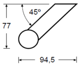
H715 \varnothing 32-332mm
